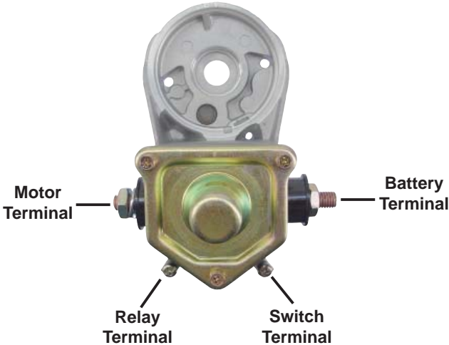
Denso OSGR Solenoid (Heavy Duty)
