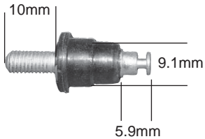
76-82168 Switch Terminal
