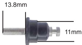
76-82131 Switch Terminal
