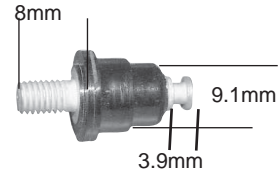
76-82130 Switch Terminal
