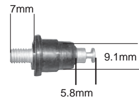
76-82130-1 Switch Terminal
